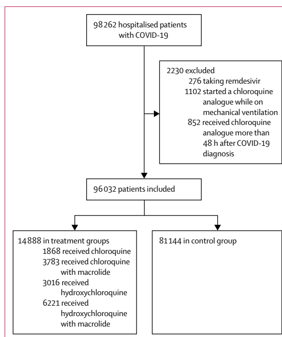
Figure 1: Study profile
